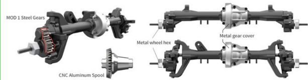
Portal axles with metal gear cover
