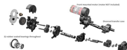
Specially arranged transfer case
